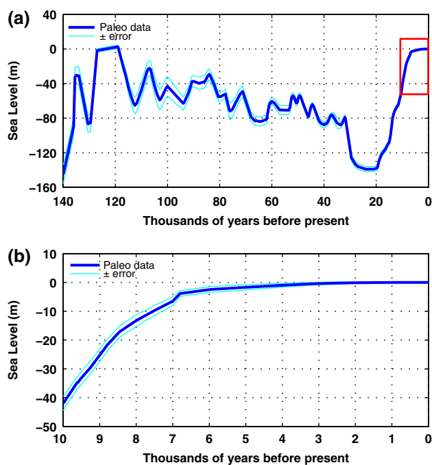
Fig. 1 Estimates of sea-level change over the last 140,000 years (Lambeck and Chappell 2001; Lambeck et al. 2002). The error bars indicate the limits of estimates from the available data and the red box in a indicates the period covered in b
