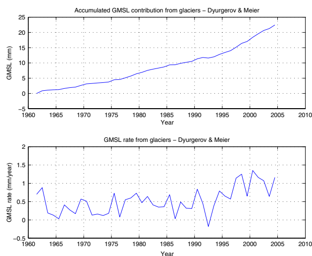
Fig. 5 Contributions from glaciers and ice caps to the global-mean sea level (Dyurgerov and Meier 2005). The lower panel is the annual contribution and the upper panel is the accumulated contribution from 1961
