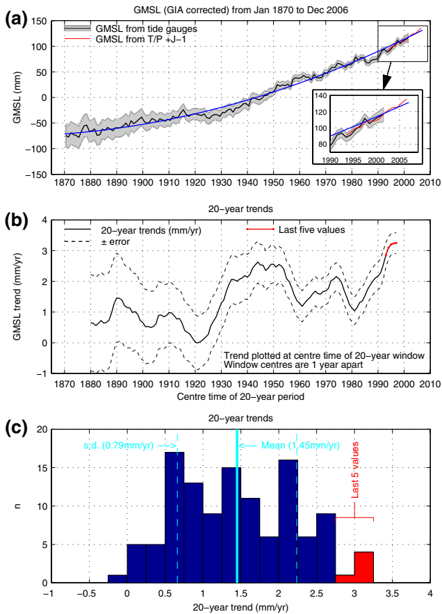
Fig. 3 a Global mean sea level from 1870 to 2006 with one standard deviation error estimates. b The linear trends in sea level over 20-year periods, with one sigma error on the trend estimates shown by the dotted lines. c The histogram of trends over the period 1870 to 2006. The mean value and one standard deviation are shown. The values for the last five 20-year periods centred on 1992 or later are shown in red in panels b and c (T/P+J-1 is the combined TOPEX/POSEIDON and Jason-1 satellite altimeter record)
