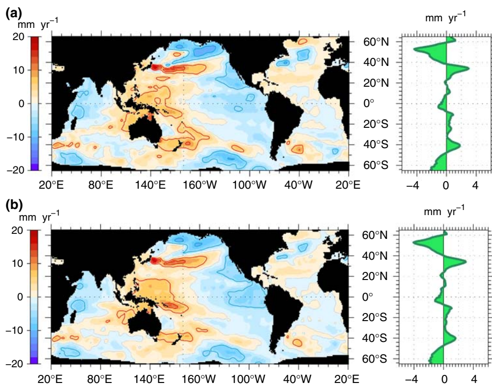
Fig. 4 a The spatial distribution of the rates of sea-level rise, plotted about the mean value for the period January 1993 to December 2003, as measured from satellite altimeter data. b The thermal expansion component for the upper 700 m, as estimated from a reduced-space optimal interpolation based on the techniques employed by Domingues et al. (2008)
