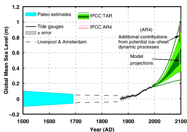
Fig. 7 Sea levels from 1500 to 2100. The blue bar indicates the range of paleo observations from Figs. 1, 2 and 3, the dotted lines from 1700 to 1860 indicate the range of sea levels inferred from Europe’s longest tide-gauge records at Amsterdam and Liverpool from Fig. 2, the dark line from 1870 to 2006 indicates the global average sea level from Fig. 3 and the curves from 1990 to 2100 are the projections from Fig. 6
