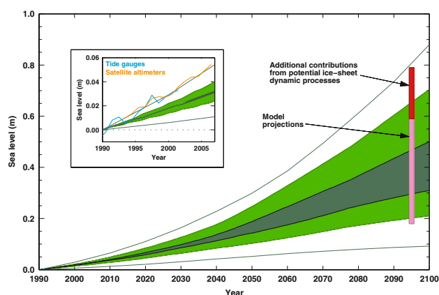
Fig. 6 Projected sea-level rise for the 21st century. The projected range of global-averaged sea-level rise from the IPCC (2001) assessment report for the period 1990–2100 is shown by the lines and shading (the dark shading is the model average envelope for all SRES greenhouse gas scenarios, the light shading is the envelope for all models and all SRES scenarios, and the outer lines include an allowance for an additional land-ice uncertainty). The updated AR4 IPCC projections (90% confidence limits) made in 2007 are shown by the bars plotted at 2095, the magenta bar is the range of model projections and the red bar is the extended range to allow for the potential but poorly quantified additional contribution from a dynamic response of the Greenland and Antarctic ice sheets to global warming. Note that the IPCC AR4 states that “larger values cannot be excluded, but understanding of these effects is too limited to assess their likelihood or provide a best estimate or an upper bound for sea-level rise.” The inset shows the 2001 projection compared with the observed rate estimated from tide gauges (blue) and satellite altimeters (orange) (based on Church et al. 2001; Meehl et al. 2007; Rahmstorf et al. 2007)
