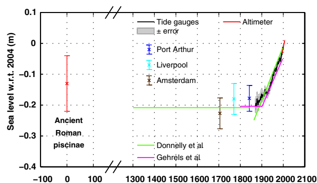
Fig. 2 Sea-level estimates from sedimentary records near New York (Donnelly et al. 2004) and Halifax (Gehrels et al. 2006) compared with the estimates of global mean sea level shown in Fig. 3. The sedimentary estimates of the sea level have been plotted with zero trend for the early part of the record. The estimated local sea level (compared with the present day local sea level and corrected for GIA [glacial isostatic adjustment]) in ancient Roman times (Lambeck et al. 2004), near the start of the tide-gauge record at Amsterdam and Liverpool (Woodworth 1999) and at the Port Arthur (Tasmania, Australia) benchmark in 1840 (Hunter et al. 2003) are shown in red, brown, light blue and dark blue, respectively. The error bars on these estimates are one standard deviation
